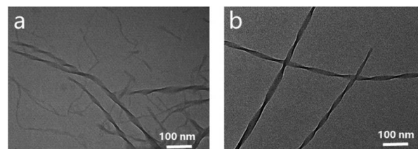
Fig. 4 TEM images of S -TPE-Ph-PEA assemblies from the DCM/HEX 1 : 9 system after self-assembling for 2 min (a) and 4 min (b), illustrating the formation and growth of helical fibers of S -TPE-Ph-PEA assemblies from solutions with a concentration of 1 \times 10^{-4} M.
