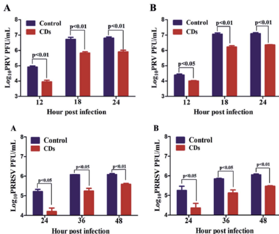
Fig. 11 The replication process of PRV (top) and PRRSV (bottom). Reproduced with permission from ref. 50. Copyright 2016 Elsevier Ltd.
