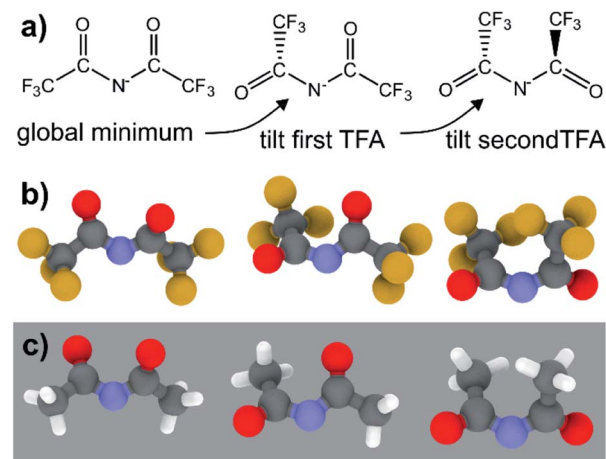
Fig. 10 (a) Schematic representation of the conformational changes in [\text{N}(\text{TFA})_2]^- , (b) the optimised minimum geometries of this anion, (c) the corresponding structures for the non-fluorinated analogue [\text{N}(\text{Ac})_2]^- .
