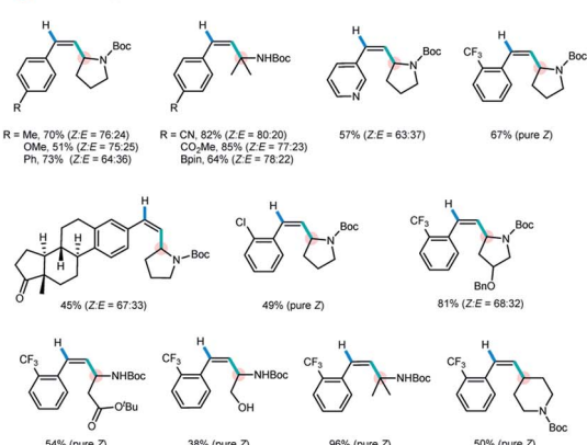
Scheme 6 Hydroalkylation of alkynes via photoredox and nickel dual catalysis.
