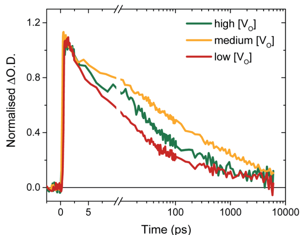
Fig. 5 Normalised ultrafast transient absorption kinetics in 0.1 M H_2SO_4 , probing the electron decay at 700 nm from \sim 200 femtoseconds to 6 ns after excitation with 355 nm ( 0.2 \text{ mJ cm}^{-2} , no bias) for 'high' to 'medium' and 'low' [V_O] doping concentrations.
