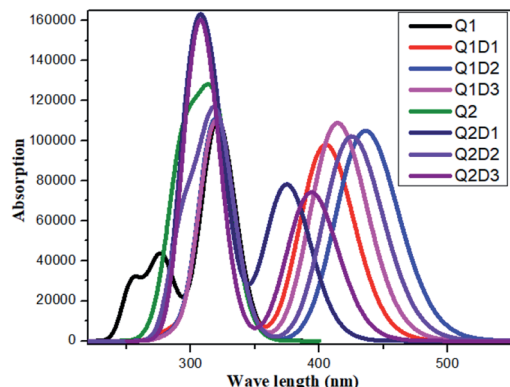
Fig. 5 Simulated absorption spectra of quinoline-carbazole based compounds (Q1, Q1D1–Q1D3, Q2, Q2D1–Q2D3).
