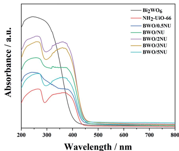
Fig. 8 UV-vis DSR spectra of as-prepared samples.
