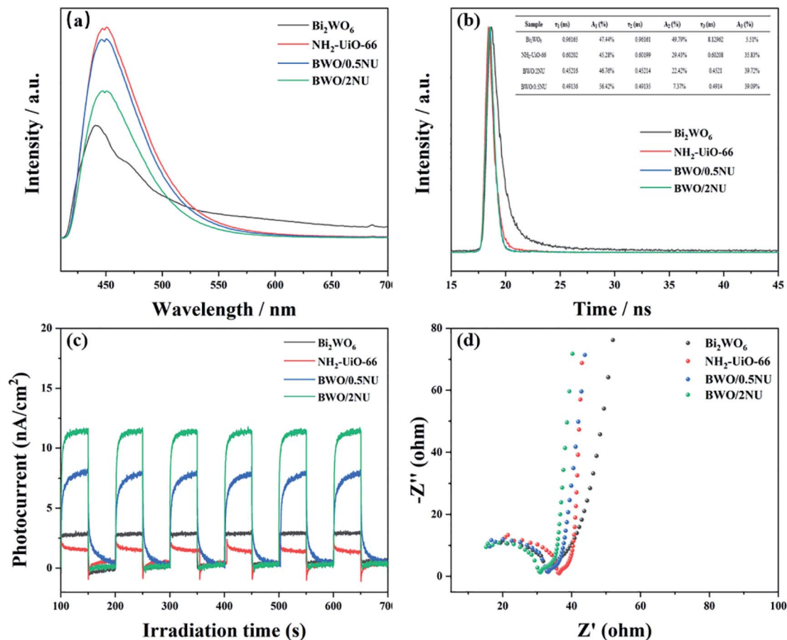
Fig. 7 (a) Stable state PL, and (b) TRPL spectra, (c) photocurrent responses, and (d) EIS images of \text{Bi}_2\text{WO}_6 , \text{NH}_2\text{-UiO-66} , \text{BWO/0.5NU} and \text{BWO/2NU} .
