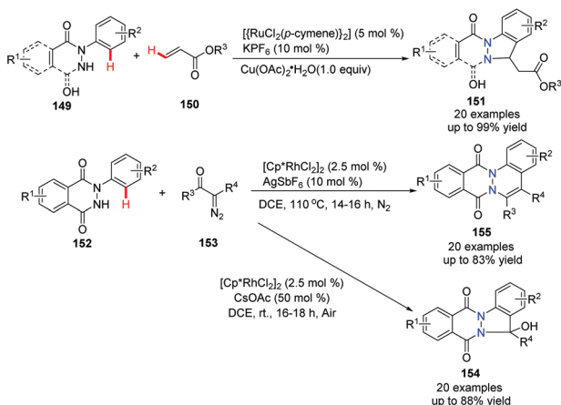
Scheme 36 \text{Ru}(\text{II}) or \text{Rh}(\text{III}) -catalyzed annulation of N -arylphthalazinedione with acrylates or diazo carbonyl compounds.
