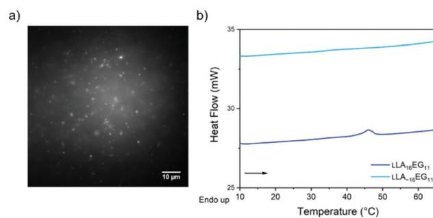
Fig. 4 (a) TIRF image of disperse \text{lLA}_{\sim 16}\text{EG}_{11} upon self-assembly in water. (b) Micro-DSC traces of \text{lLA}_{16}\text{EG}_{11} and \text{lLA}_{\sim 16}\text{EG}_{11} at 5 mg mL -1 after self-assembly in water.
