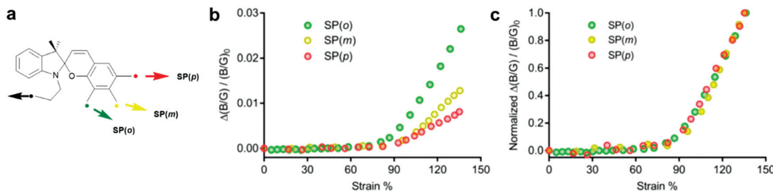
Fig. 9 (a) Spirothiopyran regioisomers with force handles in ortho -, meta - and para -position towards the spiro C–O bond. (b) Alteration of B/G intensity. (c) Alteration of B/G intensity normalized to the value at 135% strain. 221 Adapted with permission from ref. 221 Copyright 2018 American Chemical Society.
