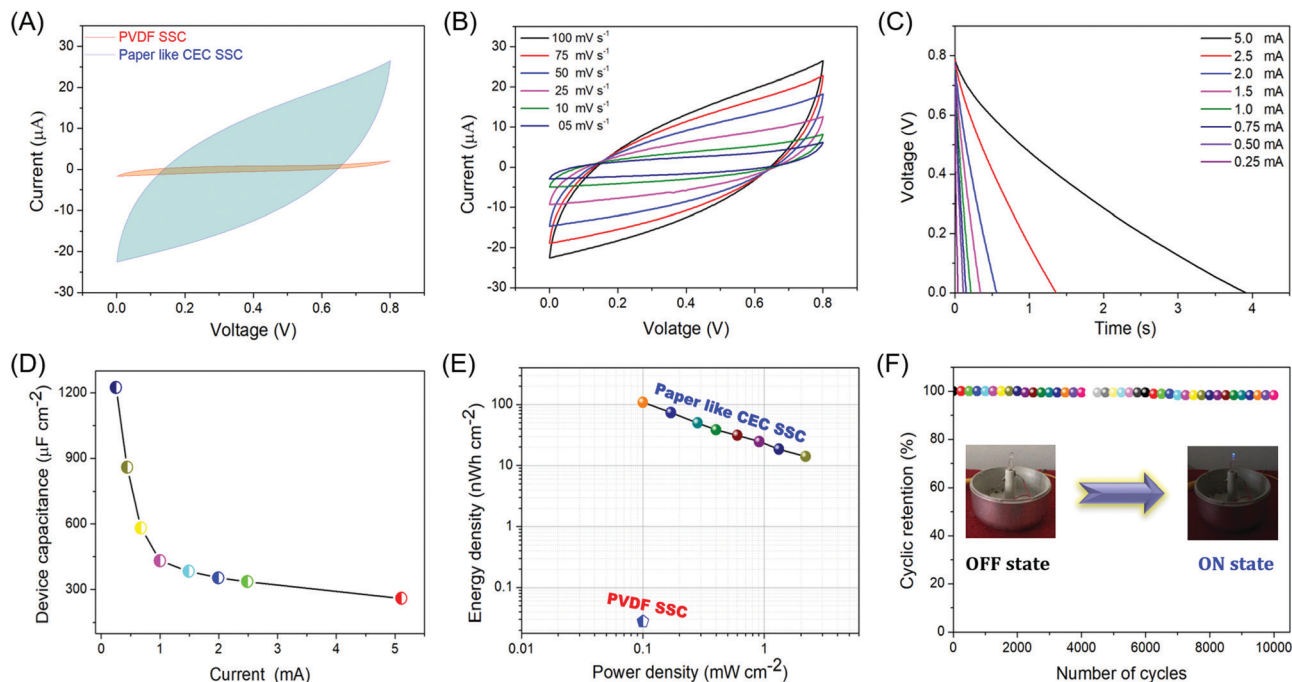
Fig. 6 Electrochemical performance of the P-CEC SSC device. (A) Relative CV profiles of the PVDF SSC and P-CEC SSC devices tested over the scan rate of 100 \text{ mV s}^{-1} , (B) CV profile of the P-CEC SSC device at different scan rates (5 to 100 \text{ mV s}^{-1} ), (C) discharge profile of the P-CEC SSC device at various currents in the range of 0.25 to 5.0 mA, (D) variation in the capacitance of the P-CEC SSC device at different currents, (E) Ragone chart of the P-CEC SSC device, and (F) cycling performance of the P-CEC SSC device over 10 000 cycles at a constant current of 1 mA.
