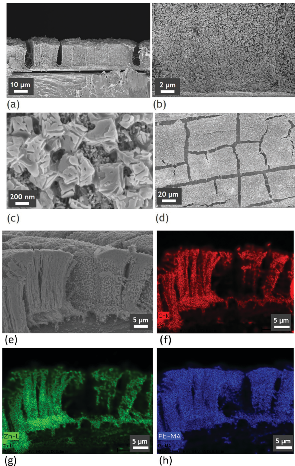
Fig. 4 (a–c) SEM cross-section views at different magnifications of Al/VACNT/ZnO/perovskites and (d) top view of the deposit. (e) SEM cross-section of Al/VACNT/ZnO/perovskite and associated EDX analysis. (f) Carbon repartition, (g) Zn repartition and (h) Pb repartition. These pictures show the efficient colocalization of CNTs, ZnO and perovskite.
