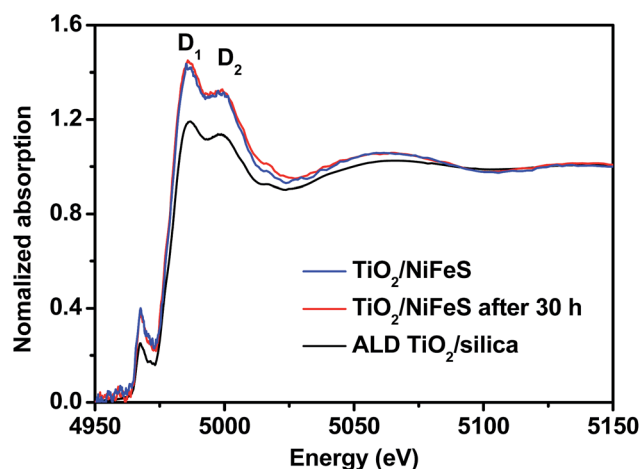
Fig. 6 Comparison of Ti K-edge X-ray absorption near edge structure (XANES) data collected on the as-prepared TiO 2 /silica and 5 nm TiO 2 /NiFeS nanosheets attached to Ni foam, before and after 30 hours of HER operation.
