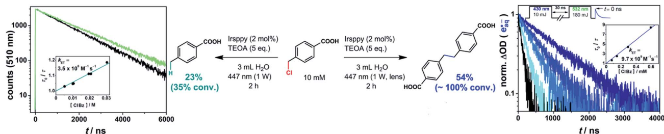
Fig. 3 ^3\text{Irspy} (left) and e_{\text{aq}}^{\cdot-} (right) induced reductive activation of 4-(chloromethyl)benzoic acid resulting in the hydrogen abstraction and the dimerization main product, respectively, together with rate constant determinations of the two substrate activation reactions. The conditions for preparative irradiation experiments are given at the equations. For further details, see text and Section 1.3 of the ESI† (which enlarges on the two-pulse experiments shown in the right part of the figure).
