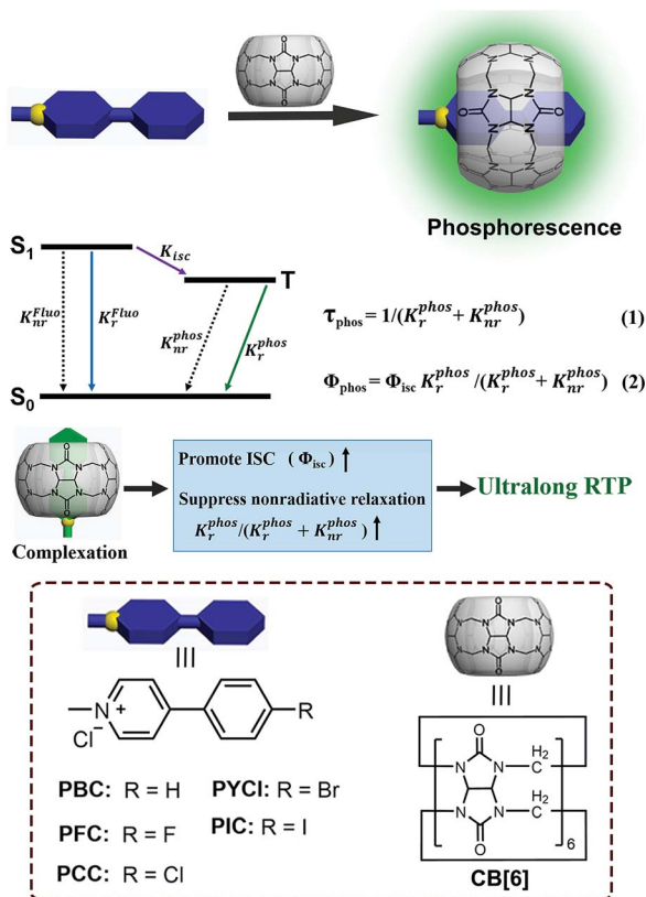
Scheme 1 Schematic illustration of the solid-state supramolecular strategy and Jablonski diagram for radiative and non-radiative processes. ( K_{Fluo}^{S_1} is the radiative rate constant of the lowest excited singlet state S_1 ; K_{Fluo}^{S_0} is the nonradiative rate constant of the lowest excited singlet state S_1 ; K_{isc} is the intersystem crossing rate constant from the excited singlet state to the triplet state; K_r^{phos} is the radiative rate constant of the lowest excited triplet state T_1 ; K_{nr}^{phos} is the nonradiative rate constant of the lowest excited triplet state T_1 ; \tau_{phos} is the lifetime of the excited triplet state; \Phi_{phos} is the quantum yield of phosphorescence; and \Phi_{isc} is the quantum yield of intersystem crossing from the excited singlet state to the triplet state; inset: the molecular structures of the guests and host).
