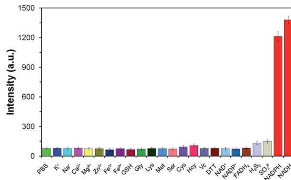
Fig. 3 Fluorescence responses of the probe TCF-MQ (10 \mu\text{M} ) for various analytes: 1 mM \text{K}^+ , \text{Na}^+ , \text{Ca}^{2+} , \text{Mg}^{2+} , \text{Zn}^{2+} , \text{Fe}^{3+} , \text{Fe}^{2+} , GSH, Gly, Lys, Met, or Ser; 100 \mu\text{M} Cys, Hcy, VC, or DTT; 5 \mu\text{M} \text{H}_2\text{S}_2 or \text{SO}_3^{2-} ; and 50 \mu\text{M} \text{NAD}^+ , \text{NADP}^+ , \text{FADH}_2 , \text{NADPH} , or \text{NADH} .
