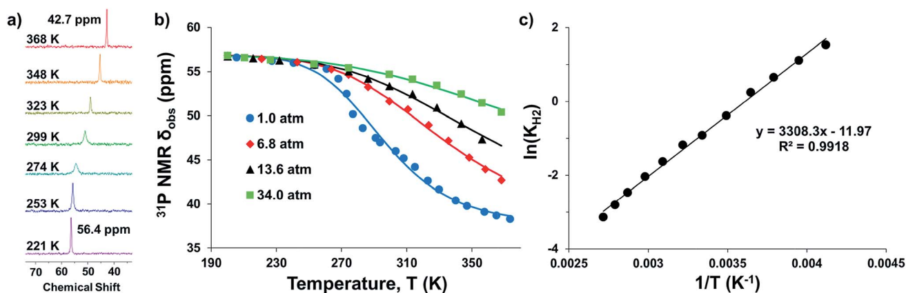
Fig. 2 (a) VT ^{31}\text{P} NMR spectra of 2 under 6.8 atm \text{H}_2 in toluene- \text{d}_8 from 368 to 221 K. (b) Plots of ^{31}\text{P} \delta vs. T obtained for various \text{H}_2 pressures. Data are shown as points, and solid traces represent the best-fit curves obtained by varying \Delta H^\circ and \Delta S^\circ as parameters (see ESI†). (c) Representative van't Hoff plot of \ln(K_{\text{H}_2}) vs. 1/T at 6.8 atm \text{H}_2 . The thermodynamic binding parameters shown in Table 2 were determined from van't Hoff plots for data sets collected at 6.8 and 13.6 atm \text{H}_2 , which exhibit fast chemical exchange.
