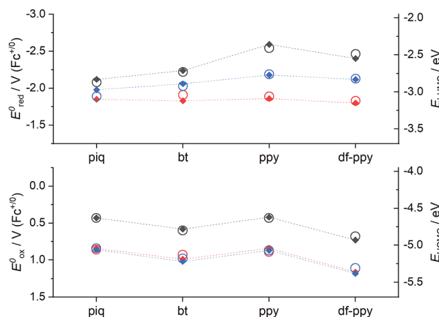
Fig. 4 Effects of ligand structure on electrochemical properties (solid diamonds; left axes) and calculated MO energies (open circles; right axes; BP86/def2-TZVP calculations), for [\text{Ir}(\text{C}^{\text{N}})_2(\text{acac})] (grey symbols), [\text{Ir}(\text{C}^{\text{N}})_2(\text{dm-bpy})]^+ (red symbols), and [\text{Ir}(\text{C}^{\text{N}})_2(\text{ptb})]^+ (blue symbols) complexes, where \text{C}^{\text{N}} = \text{piq} , \text{bt} , \text{ppy} , or \text{df-ppy} . The upper graph shows reduction potentials and LUMO energies, and the lower graph shows oxidation potentials and HOMO energies.
