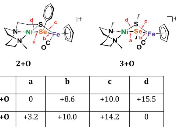
Fig. 6 Relative energies of oxygenated isomers of N 2 SSePh model, 2+O , and the bidentate, separated donors in the N 2 SMeSeMe model, 3+O , in kcal mol -1 . A range of functionals and basis sets were explored and found to elicit minor differences on energies of complexes but do not change the ordering of isomers' energies (Fig. S41†).
