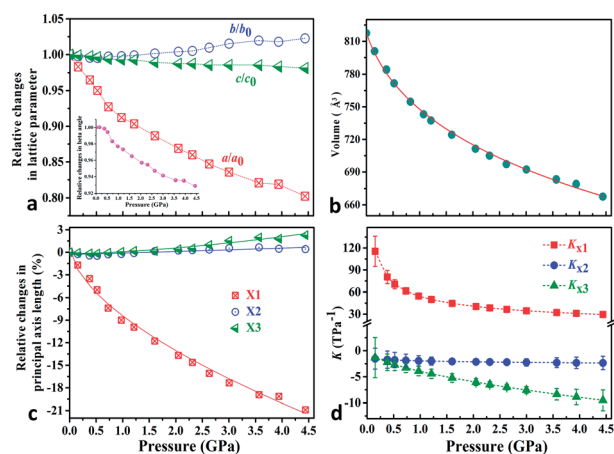
Fig. 2 (a) Relative changes of lattice parameters as a function of pressure; the \beta angle changes are shown as an inset in (a). (b) The third order Birch–Murnaghan EoS fits 31 for cell volume vs. pressure (Fig. S3†). (c) Pressure-dependent relative changes in length for the three principal axes and (d) the corresponding principal compressibility K_{X1} , K_{X2} and K_{X3} .
