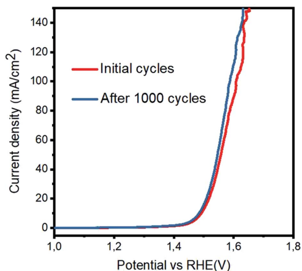
Fig. 6 Durability experiment via cyclic voltammetry at the scan rate of 20 mV s -1 after 2000 cycles in 1 M KOH.
