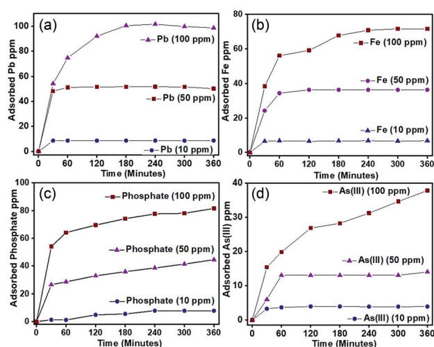
Fig. 7 Kinetic study of ions (a) Pb 2+ , (b) Fe 3+ , (c) PO 4 3− and (d) AsO 2 1− at their initial concentration of 10, 50 and 100 ppm with time.
