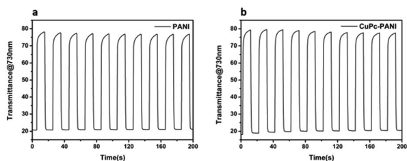
Fig. 7 Kinetic optical transmittance curves at 730 nm of (a) pure PANI and (b) the CuPc-PANI composite film, each subjected to switching between -0.2 and 0.7 V for 10 s at each step in an aqueous solution of 1 M H 2 SO 4 .
