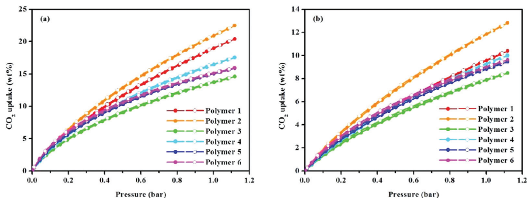
Fig. 4 (a) Volumetric CO₂ adsorption isotherms and desorption isotherms up to 1.13 bar at 273.15 K, and (b) volumetric CO₂ adsorption isotherms and desorption isotherms up to 1.13 bar at 298.15 K.
