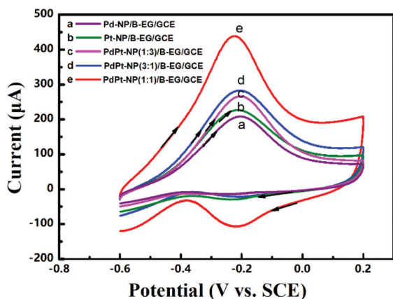
Fig. 6 Cyclic voltammograms of 0.05 M methanol in 1.5 M KOH at a scan rate of 100 mV s -1 on a Pd-NP(30%)/B-EG/GCE (a), a Pt-NP(30%)/B-EG/GCE (b), a PdPt-NP(1:3)/B-EG/GCE (c), a PdPt-NP(3:1)/B-EG/GCE (d), and a PdPt-NP(1:1)/B-EG/GCE (e).
