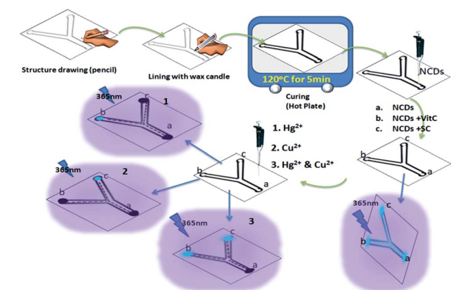
Scheme 2 Fabrication of filter paper based microfluidic detection device and detection of \text{Hg}^{2+} and \text{Cu}^{2+} with NCDs (Vit C = vitamin C; SC = trisodium citrate).
