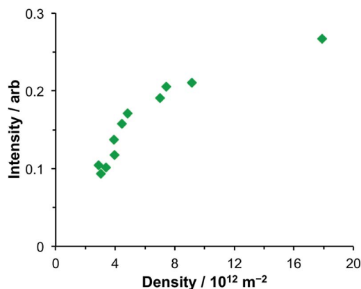
Fig. 5 Variation in the intensity of the feature at 1.43 eV in the extinction spectra of nanostructure arrays coupled to LHCII as a function of the density of nanostructures in the array.
