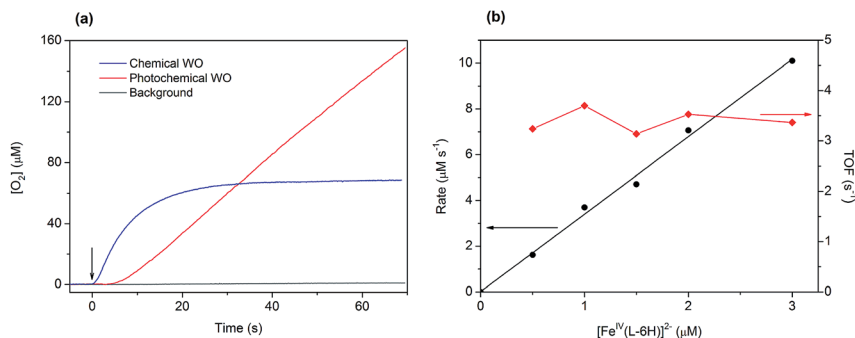
Fig. 3 (a) Traces of oxygen evolution obtained in photochemical (red trace: [\text{Fe}^{\text{IV}}(\text{L-6H})]^{2-} ( 1\text{ }\mu\text{M} ), [\text{Ru}(\text{bpy})_3]^{2+} ( 0.2\text{ mM} ) and \text{S}_2\text{O}_8^{2-} ( 2\text{ mM} )) and chemical water oxidation experiments (blue trace: [\text{Fe}^{\text{IV}}(\text{L-6H})]^{2-} ( 1.5\text{ }\mu\text{M} ) and [\text{Ru}(\text{bpy})_3]^{3+} ( 1\text{ mM} )). Oxygen evolution in the absence of catalyst is given for comparison (grey trace: [\text{Ru}(\text{bpy})_3]^{2+} ( 0.2\text{ mM} ) and \text{S}_2\text{O}_8^{2-} ( 2\text{ mM} )). The arrow indicates the beginning of the reaction (the start of illumination or addition of the oxidant, respectively). (b) Initial water oxidation rates (circles) and TOF (diamonds) as a function of the catalyst concentration for chemical water oxidation using [\text{Ru}(\text{bpy})_3]^{3+} ( 1\text{ mM} ).
