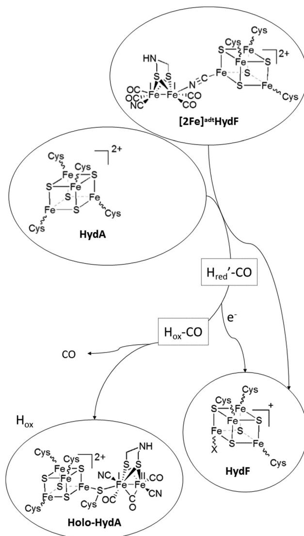
Scheme 1 Schematic representation of H-cluster assembly. The transfer of the pre-catalyst ( [2\text{Fe}]^{\text{JadT}} ) from HydF results in the release of a CO ligand and oxidation of the dinuclear complex to give \text{H}_{\text{ox}} ( [\text{Fe}^{\text{II}}\text{Fe}^{\text{I}}] \cdot [\text{4Fe4S}]^{2+} \cdot \text{HydA} ), with concomitant reduction of the [\text{4Fe4S}] cluster on HydF ( [\text{4Fe4S}]^+ \cdot \text{HydF} ). Note that the model for [2\text{Fe}]^{\text{JadT}} binding to HydF is based on ref. 5. An alternative model, with a reversed \mu\text{-CN}^- bond is proposed in ref. 27.
