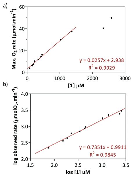
Fig. 3 a) Plot of maximum rate of O_2(g) evolution determined at 20% conversion of CAN vs. concentration of catalyst [\text{Cp}^*\text{IrCl}(\text{Melm})_2\text{CHCOO}] (1). b) Log(rate)-log[1] plot and the corresponding linear fit.
