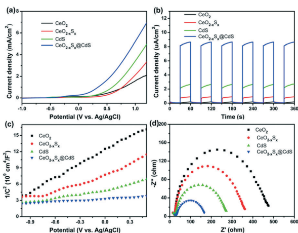
Fig. 5 (a) Linear sweep voltammetry and (b) photocurrent response measurements of the \text{CeO}_2 , \text{CeO}_{2-x}\text{S}_x , CdS and \text{CeO}_{2-x}\text{S}_x/\text{CdS} samples under visible-light irradiation ( \lambda > 420 \text{ nm} ) and at a voltage of 0.4 V. (c) Mott-Schottky plots and (d) EIS Nyquist plots of the \text{CeO}_2 , \text{CeO}_{2-x}\text{S}_x , CdS and \text{CeO}_{2-x}\text{S}_x/\text{CdS} samples.
