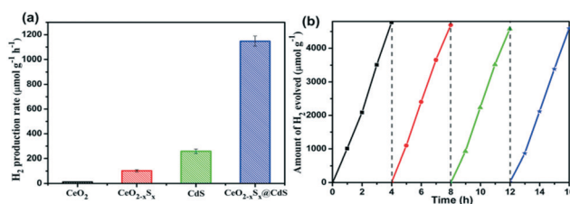
Fig. 6 (a) Comparison of the \text{H}_2 evolution rate of \text{CeO}_2 , \text{CeO}_{2-x}\text{S}_x , CdS and \text{CeO}_{2-x}\text{S}_x/\text{CdS} photocatalysts and (b) stability test of \text{H}_2 evolution for \text{CeO}_{2-x}\text{S}_x/\text{CdS} under visible-light irradiation ( \lambda > 420 \text{ nm} ).
