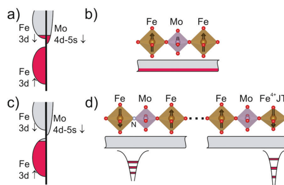
Fig. 1 (a) Schematic band filling of \text{Sr}_2\text{FeMoO}_6 . The Fermi level is nearby the bottom of \text{Fe-3d}_{t2g}\downarrow-\text{Mo-(4d,5s)}\downarrow bands. (b) In the oxide \text{FeO}_6 and \text{MoO}_6 octahedra are regular (top sketch) and the free carriers in the conduction band (bottom sketch) promote long range ferromagnetic order. (c) Schematic band filling of \text{Sr}_2\text{FeMoO}_{4.9}\text{N}_{1.1} . The oxidation of cations induced by N reduces the total number of electrons, and the filling of the bands. In the nitrated sample, the Fermi level shifts down to the top of the \text{Fe-3d}\uparrow band. (d) Localized states formed around defect-related potential wells (e.g.: nitride sites, Jahn–Teller \text{Fe}^{4+} ions) that trap electrons, hindering carrier mobility, weakening double exchange ferromagnetic interactions and cancelling long range ordering.
