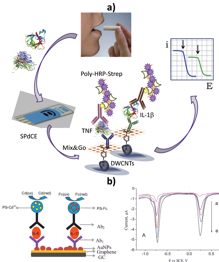
Fig. 16 Multiplexed electrochemical sandwich immunoplatforms using (a) multielectrode arrays or (b) barcode configurations. Simultaneous amperometric determination of TNF and IL-1β at a SPdCE modified with 4-carboxyphenyl-functionalized double-walled carbon nanotubes (HOOC-Phe-DWCNTs) and polymeric coating Mix&Go to immobilize the capture antibodies in an oriented manner (a). Schematic illustration of the bioplatfrom developed for the simultaneous SWV determination of IL-6 and IL-17 using polystyrene spheres (PS) containing Cd 2+ or ferrocene (Fc) as tags (b, left). SWV traces recorded for simultaneous determination of increasing concentrations of IL-6 and IL-17 standards (b, right; from (a) to (e): 5, 50, 100, 500, 1000 pg mL -1 ). Reproduced and adapted from (a) ref. 19 and (b) ref. 184 with permission.
