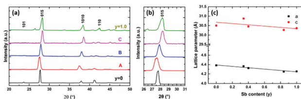
Fig. 8 (a) Grazing incidence XRD patterns from 3 positions (A–C; Sb poor to Sb rich) of a ternary sample deposited from a 1:1 ratio of [\text{SbCl}_3(\text{Te}^n\text{Bu}_2)_3] and [\text{BiCl}_3(\text{Te}^n\text{Bu}_2)_3] , together with the binary phases ( \text{Sb}_2\text{Te}_3 and \text{Bi}_2\text{Te}_3 ). Position A: a = 4.370(11) and c = 30.80(8) Å, position B: a = 4.327(8) and c = 30.54(8) Å, position C: a = 4.249(9) and c = 30.29(8) Å. (b) Expanded XRD patterns showing the systematic shift of the 015 peak; (c) refined lattice parameters as a function of the Sb content for different as-deposited (\text{Bi}_{1-y}\text{Sb}_y)_2\text{Te}_3 films.
