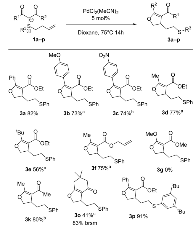
Scheme 5 Scope of dihydrofurans. a Reactions were carried out at 55 °C for 14 h. b Reactions were carried out at 75 °C for 72 h. c Reactions were carried out at 55 °C for 72 h.
