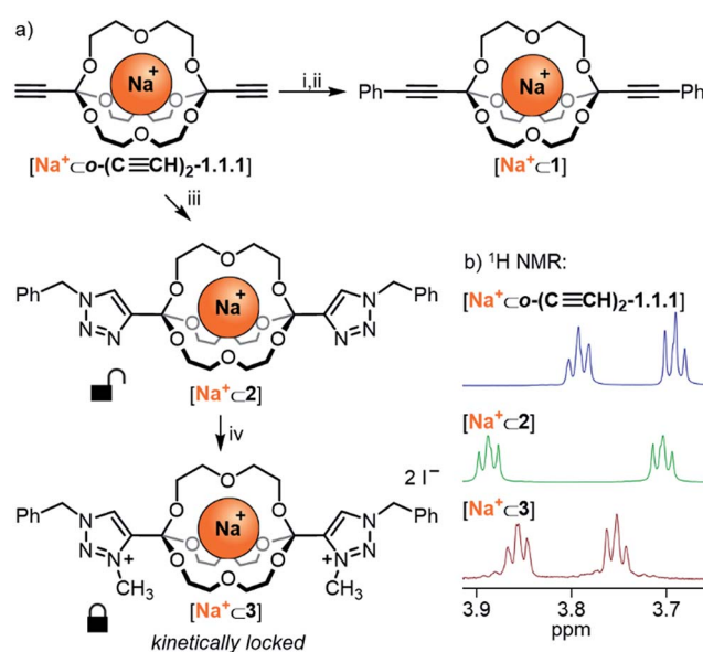
Scheme 3 Post-functionalization of orthoester cryptands. (a) Reaction conditions: (i) [ Na + ⊂ o-(C≡CH) 2 -1.1.1 ] (11.8 μmol, 1.0 equiv.), iodobenzene (23.6 μmol, 2.0 equiv.), NEt 3 (35.4 μmol, 3.0 equiv.), CuI (0.12 μmol, 0.01 equiv.), Pd(PPh 3 ) 4 (0.12 μmol, 0.01 equiv.), THF, 40 °C, 4 d, 94%. (ii) 1 (9.28 μmol, 1.0 equiv.), NaBARf (9.28 μmol, 1.0 equiv.), CH 3 CN, r.t., 5 min, quant. (iii) [ Na + ⊂ o-(C≡CH) 2 -1.1.1 ] (11.0 μmol, 1.0 equiv.), benzyl azide (22.0 μmol, 2.0 equiv.), Cu(MeCN) 4 PF 6 (0.11 μmol, 0.01 equiv.), TBTA (0.11 μmol, 0.01 equiv.), MeOH, 70 °C, 24 h, 92%. (iv) [ Na + ⊂ 2 ] (3.9 μmol, 1.0 equiv.), MeI (excess), MeCN, 70 °C, 3 d, 83%. (b) Partial 1 H NMR stacked plot (500 MHz, 298 K, CD 3 CN).
