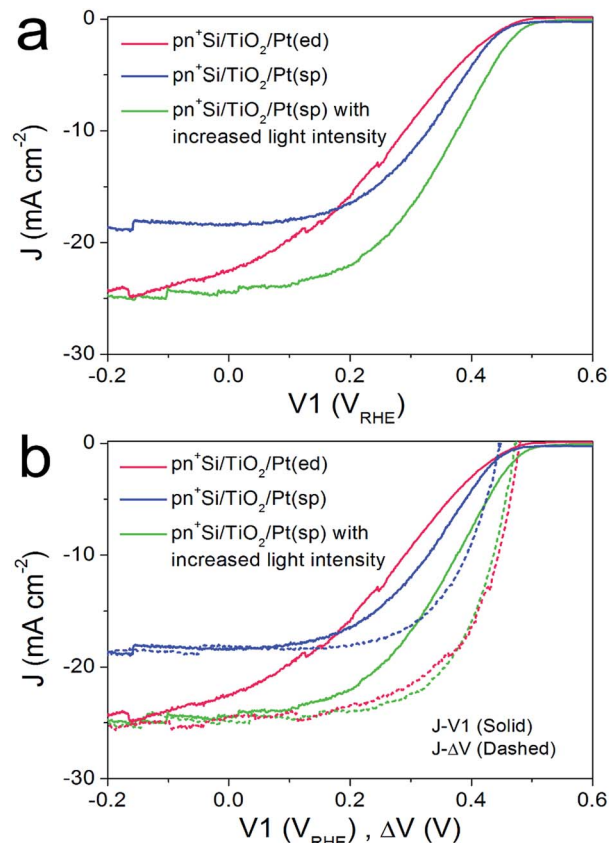
Fig. 3 (a) Comparison of J - V_1 curves between \text{pn}^+\text{Si}/\text{TiO}_2/\text{Pt}(\text{ed}) and \text{pn}^+\text{Si}/\text{TiO}_2/\text{Pt}(\text{sp}) , collected by a LSV scan with a scan rate of 10 mV s -1 towards negative potential in 0.5 M H 2 SO 4 . (b) J - \Delta V curves (dashed) of \text{pn}^+\text{Si}/\text{TiO}_2/\text{Pt}(\text{ed}) and \text{pn}^+\text{Si}/\text{TiO}_2/\text{Pt}(\text{sp}) , combined with their J - V_1 curves (solid). All data are collected under illumination. For comparison, the performance of \text{pn}^+\text{Si}/\text{TiO}_2/\text{Pt}(\text{sp}) with similar photocurrent densities as \text{pn}^+\text{Si}/\text{TiO}_2/\text{Pt}(\text{ed}) , by increasing the light intensity, is also displayed (green solid and dashed curves).
