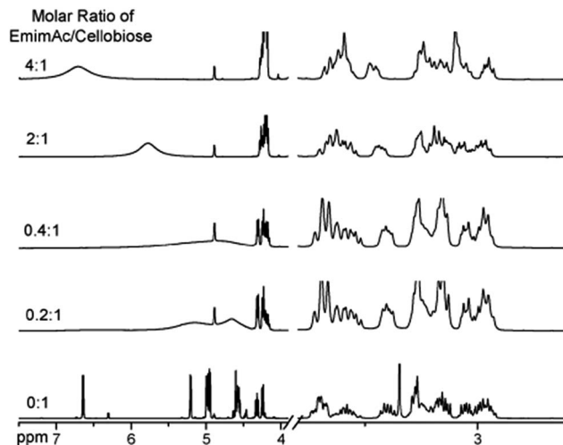
Fig. 4 Effects of different ratios of [Emim][OAc] /cellobiose on the nuclear magnetic peak in the 1 H NMR spectra of cellobiose. 49 Reproduced from ref. 49 with permission from the PCCP Owner Societies.
