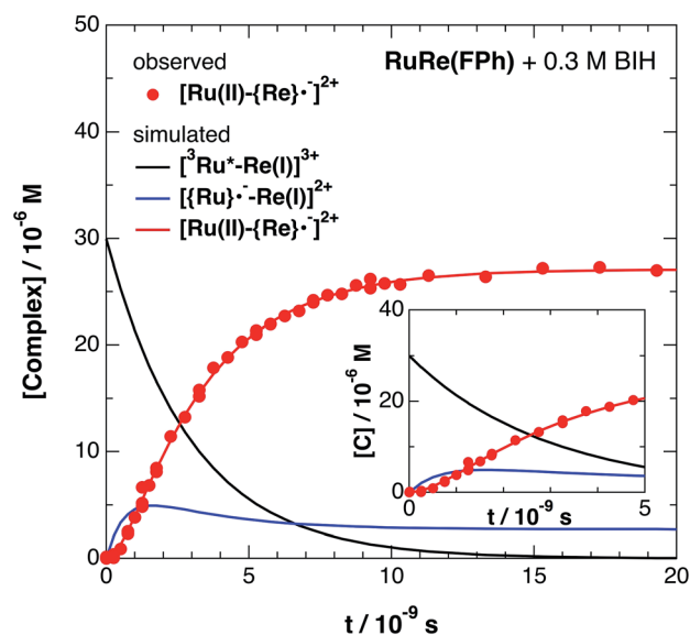
Fig. 7 Time profile of [\text{Ru(II)}-\{\text{Re}\}^{\cdot-}]^{2+} (●) in the ps-TRIR measurement of \text{RuRe(FPh)} in the presence of 0.3 M BIH in an argon-saturated DMF-TEOA (5 : 1 v/v) solution after 532 nm excitation. The kinetic simulation results for [^3\text{Ru}^*-\text{Re(I)}]^{3+} , [\{\text{Ru}\}^{\cdot-}-\text{Re(I)}]^{2+} , and [\text{Ru(II)}-\{\text{Re}\}^{\cdot-}]^{2+} are also shown (solid lines).
