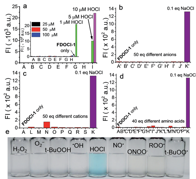
Fig. 3 Fluorescence intensity of FDOCI-1 (10 \mu\text{M} in 10 mM PBS, pH 7.2) at 686 nm after (a) adding various ROS/RNS (from (A) to (H)): \text{H}_2\text{O}_2 , \text{O}_2^{\cdot-} , t -BuOOH, \cdot\text{OH} , NO, \text{ONOO}^- , \text{ROO}^{\cdot} and t -BuOO \cdot with concentrations of 25, 50 and 100 \mu\text{M} and (I): HOCl with a concentration of 1, 5 and 10 \mu\text{M} ; the inset shows magnified data comparing A to H with 1 \mu\text{M} HOCl, (b) adding various anions (from (A') to (K')): blank, \text{CH}_3\text{COO}^- , \text{CO}_3^{2-} , \text{SO}_4^{2-} , \text{Cl}^- , \text{ClO}_4^- , \text{F}^- , \text{I}^- , \text{NO}_2^- , \text{S}_2\text{O}_3^{2-} and \text{OCl}^- , (c) adding various cations (from (L) to (S)): \text{Al}^{3+} , \text{Ca}^{2+} , \text{Cu}^{2+} , \text{Fe}^{3+} , \text{K}^+ , \text{Mg}^{2+} , \text{NH}_4^+ and \text{Ni}^+ and (d) adding various amino acids (from (B'') to (P'')): Leu, Pro, Gly, Gln, Glu, Met, Lys, Trp, Ser, Thr, Asp, Ile, Val, His and Ala). (e) Colour changes of FDOCI-1 (10 \mu\text{M} ) after adding HOCl (25 \mu\text{M} ) and other different ROS/RNS (100 \mu\text{M} ) with \lambda_{\text{ex}} = 620 nm.
