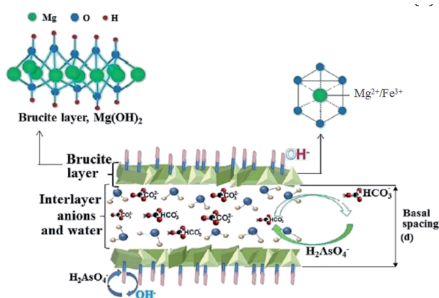
Fig. 9 Schematic mechanism of \text{As(V)} adsorption on \text{Mg-Fe-CO}_3^{2-} LDHs. 197
