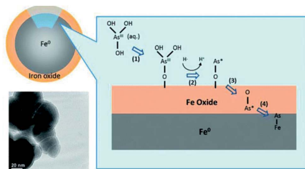
Fig. 8 The schematic diagram of the adsorption of \text{As(III)} species on nZVI particles. 200
