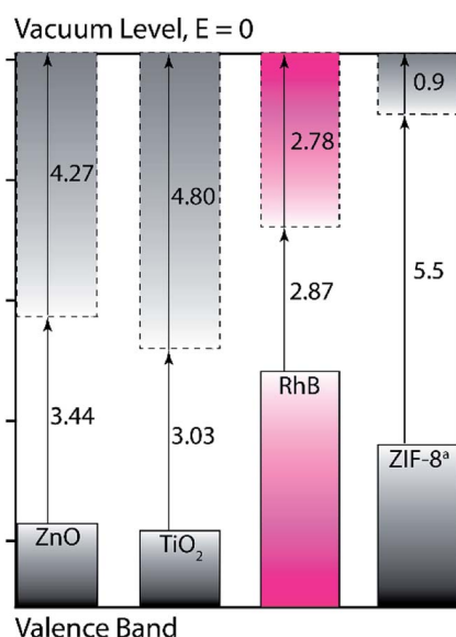
Scheme 2 Comparison of calculated electronic energy levels of RhB, ZIF-8, ZnO, and rutile \text{TiO}_2 (in eV respect to vacuum level). Dash and solid boxes represent conduction band and valence band, respectively. a Values were taken from DFT calculations with periodic boundary conditions. 64 The values for ZnO and \text{TiO}_2 are taken from previously reported DFT predicted bandgap. 70,71
