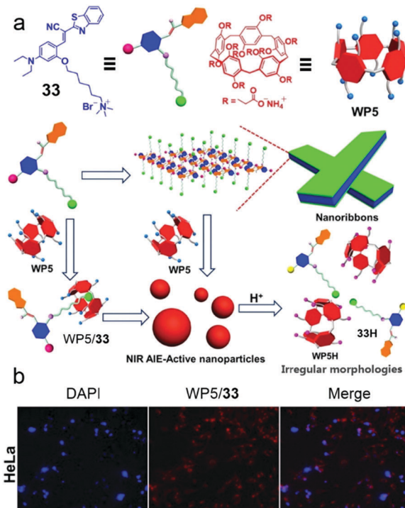
Fig. 26 (a) Schematic representation of self-assembly processes of 33 and WP5/ 33 . (b) CLSM images of HeLa cells demonstrating the cell image capability of the WP5/ 33 supra-amphiphile. Adapted with permission from ref. 101. Copyright 2016 American Chemical Society.
