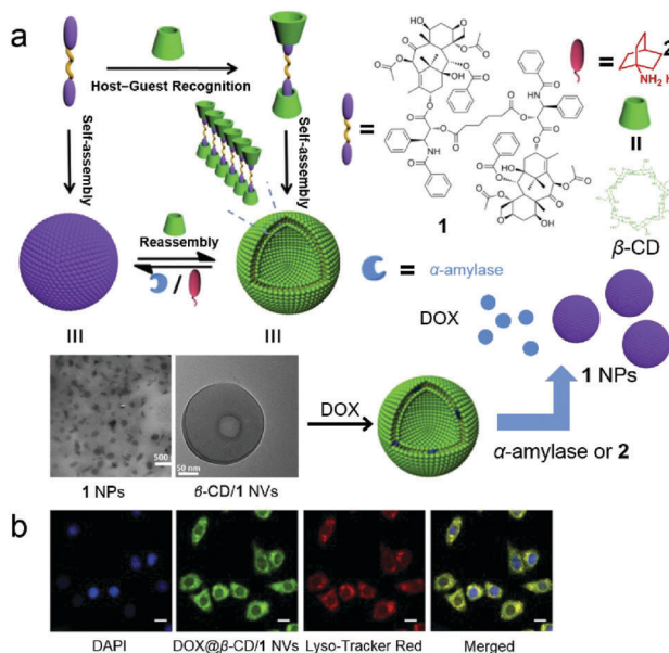
Fig. 3 (a) Schematic representation of the formation of vesicles for controlled release. (b) Confocal laser scanning microscopy (CLSM) images of HepG2 cells incubated with DOX@ \beta -CD/ 1 nanovesicles. Adapted with permission from ref. 26. Copyright 2017 American Chemical Society.
