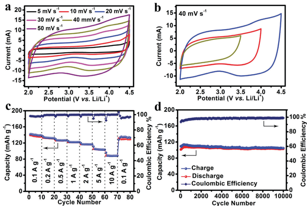
Fig. 4 Lithium storage performance of the NS-DPC cathode tested in a \text{LiPF}_6 electrolyte: (a) CV curves of the NS-DPC cathode at different scan rates. (b) CV curves of the NS-DPC cathode cycled within different potential windows at 40 \text{ mV s}^{-1} . (c) Rate performance of a NS-DPC cathode. (d) Cycling stability of a NS-DPC cathode at a current density of 5 \text{ A g}^{-1} .
