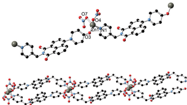
Fig. 4 (top) The structure of the repeat unit of complex 2 with labelling scheme for coordinating atoms; (bottom) extended structure of complex 2 showing the interactions between adjacent chains. Hydrogen atoms, nitrate anion disorder and lattice solvent molecules are omitted for clarity.
