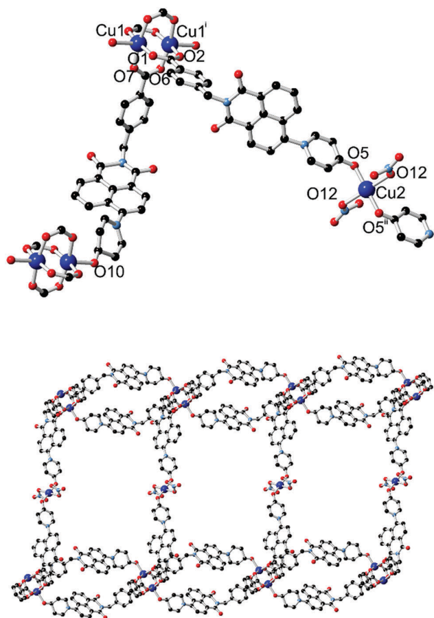
Fig. 6 (top) The two distinct copper coordination environments within the structure of 4 , with labelling scheme for coordinating heteroatoms. (bottom) Extended structure of a single layer of 4 , consisting of linear bridges between looped L2 -paddlewheel chains. Hydrogen atoms and backbone disorder are omitted for clarity. Symmetry codes used to generate equivalent atoms: (i) 1/2 - x, 3/2 - y, 1 - z ; (ii) 2 - x, 1 - y, 2 - z .
