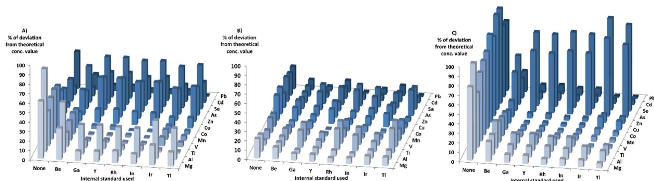
Fig. 2 Highest absolute deviation from theoretic concentration values for all matrix compositions in KED-mode, when using 1% HNO 3 -matrix for calibration. Scale restricted to a maximum of 100% deviation. (A) HNO 3 , (B) PBS, (C) Triton.
