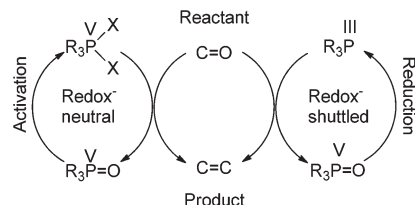
Scheme 15 General approaches to phosphorus catalysis.
