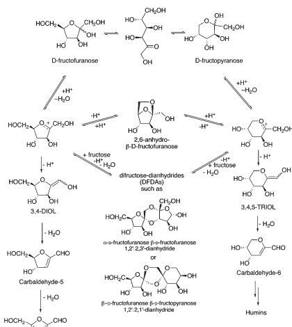
Scheme 41 Proposed intermediates of the acid-catalyzed dehydration of D-fructose to 5-HMF via a cyclic pathway, adapted with permission from ref. 171. Copyright 2012 of the Royal Society of Chemistry.
