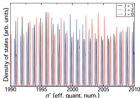
Fig. 6 Progression of heavy Rydberg resonances around the principal quantum number n = 2000 for J = 0, 1 and 2 . These states have classical turning points at around R_{tp} = 8700 a.u.
