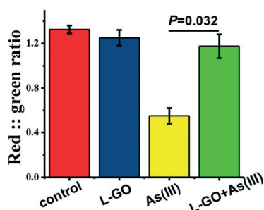
Fig. 5 Oxidative stress response to K-medium, L-GO, As(III) and concurrent exposure to L-GO and As(III). (A) TEM images of C. elegans after exposure to K-medium, L-GO, As(III), or both. Red arrows indicate mitochondria. (B) Mitochondrial membrane potential indicated by JC-1 specific fluorescence; worms were treated with K-medium, L-GO, As(III), or both. (C) The global ROS production was quantified using CM-H 2 DCFDA. (D) Average number of germline apoptotic cells induced by exposure to K-medium, L-GO, As(III) or both in wild type and mutant mev-1(kn1) strains. Results are means \pm S.D. of triplicate values ( n = 3 ) from three representative experiments.
