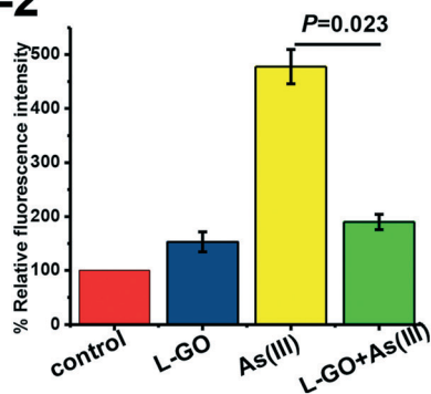
Fig. 5 Oxidative stress response to K-medium, L-GO, As(III) and concurrent exposure to L-GO and As(III). (A) TEM images of C. elegans after exposure to K-medium, L-GO, As(III), or both. Red arrows indicate mitochondria. (B) Mitochondrial membrane potential indicated by JC-1 specific fluorescence; worms were treated with K-medium, L-GO, As(III), or both. (C) The global ROS production was quantified using CM-H 2 DCFDA. (D) Average number of germline apoptotic cells induced by exposure to K-medium, L-GO, As(III) or both in wild type and mutant mev-1(kn1) strains. Results are means \pm S.D. of triplicate values ( n = 3 ) from three representative experiments.
